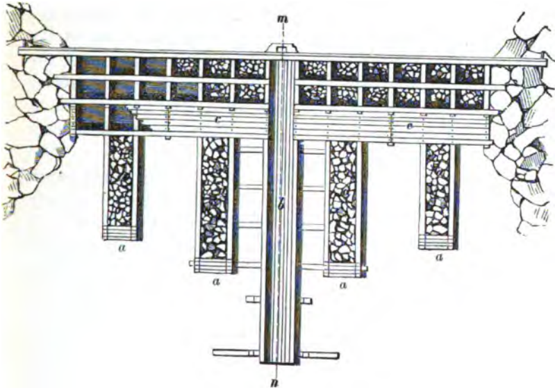
Fig. 231.—The Martin's dam in the Bavarian-Bohemian Forest, that has now been rebuilt in masonry.
